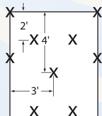
1.75 staples/yd 2 2:1 SLOPES
